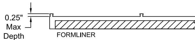
FORMLINER DETAIL
