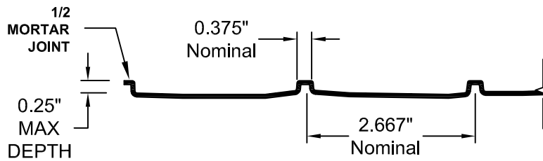
FORMLINER DETAIL
