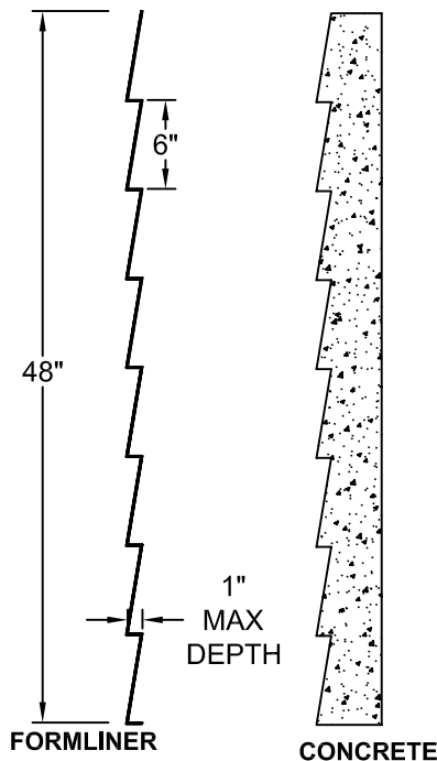
SECTION A-A FORMLINER DETAIL
