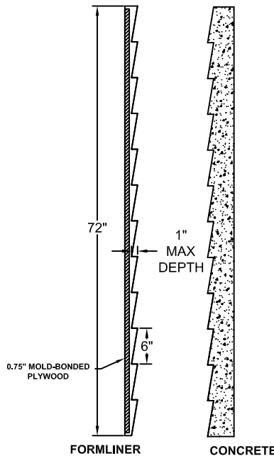
SECTION A-A FORMLINER DETAIL
