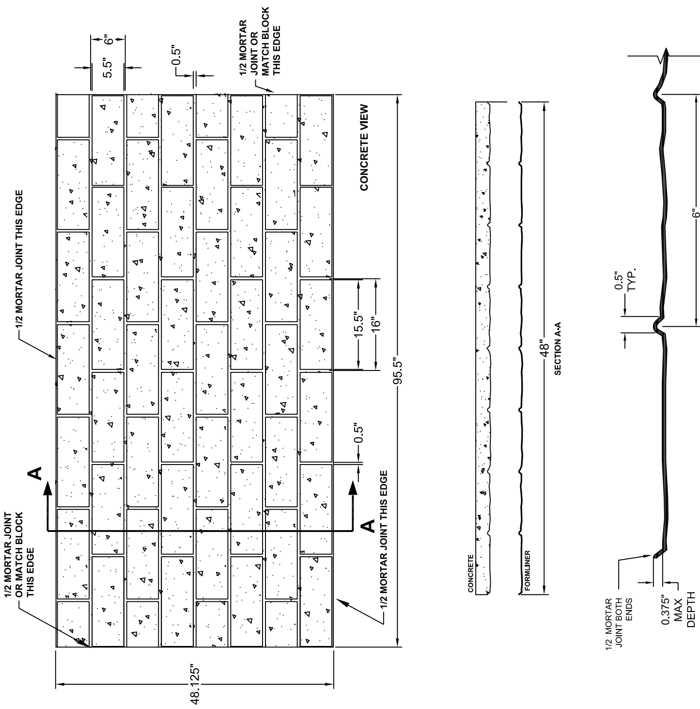
FORMLINER DETAIL
