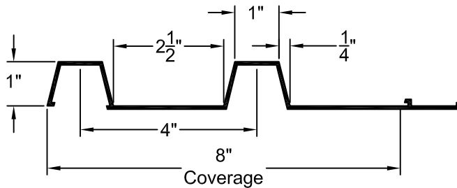
FORMLINER DETAIL
